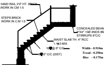
STAIRCASE DETAILS
