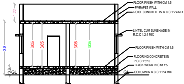
SECTION ON AA
