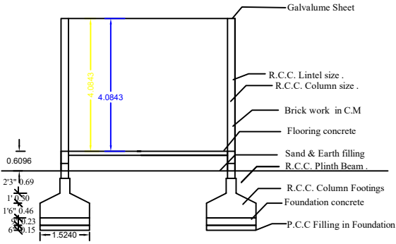
SECTION ON-AA
