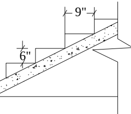
Staircase Detail Not To Scale
