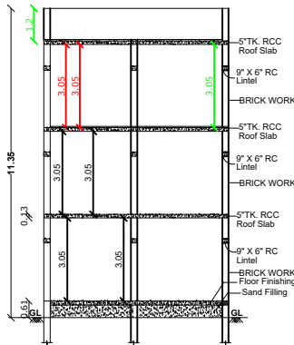
SECTION ON S-R
