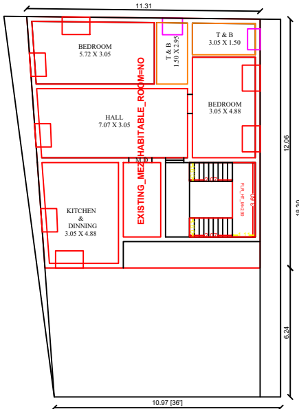
EXISTING GROUND FLOOR
