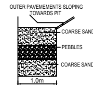
RAIN WATER PERCOLATION BED
