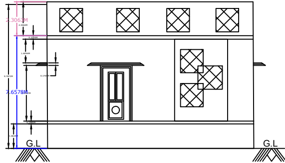
FRONT ELEVATION
