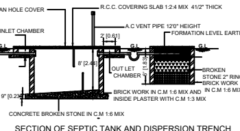
SECTION OF SEPTIC TANK AND DISPERSION TRENCH
