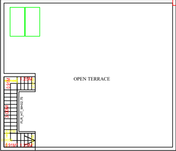
SITE PLAN
