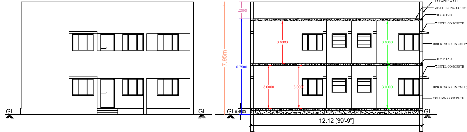
FRONT ELEVATION
