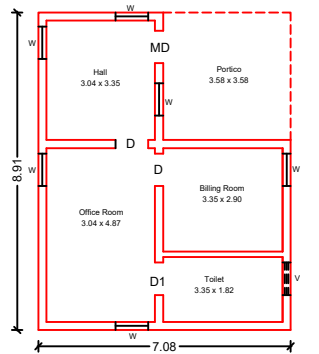
PRO.GROUND FLOOR PLAN
