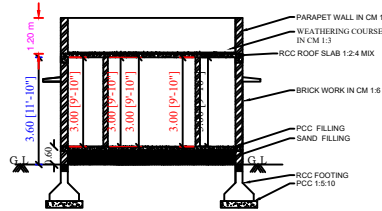
SECTION-"SR"
