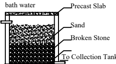
Section of Filter Unit
