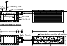
ULS OF SEPTIC TANK & DISPERSION TRENCH
