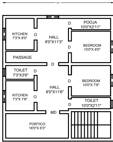
EXT. FIRST FLOOR PLAN
