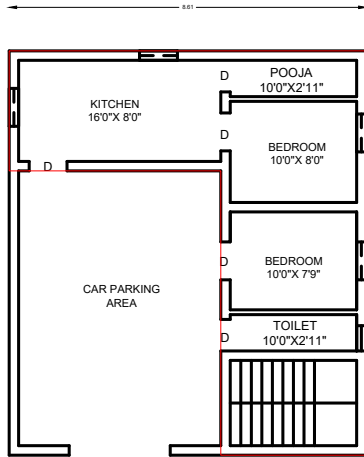
EXT. GROUND FLOOR PLAN
