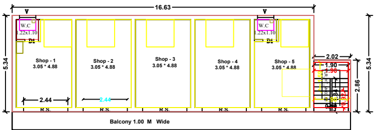
PLAN - Proposed Ground Floor - Shop
