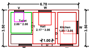
PLAN - Proposed Ground Floor Residential
