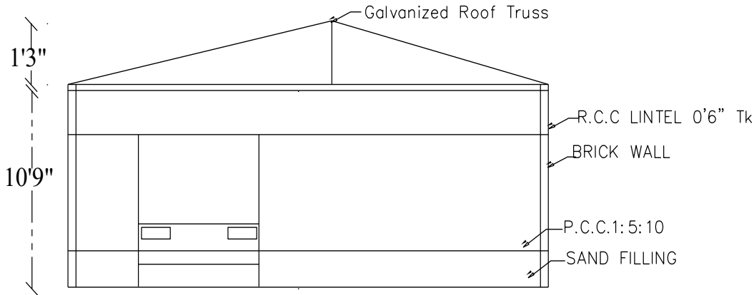
SECTION ON"AB"
