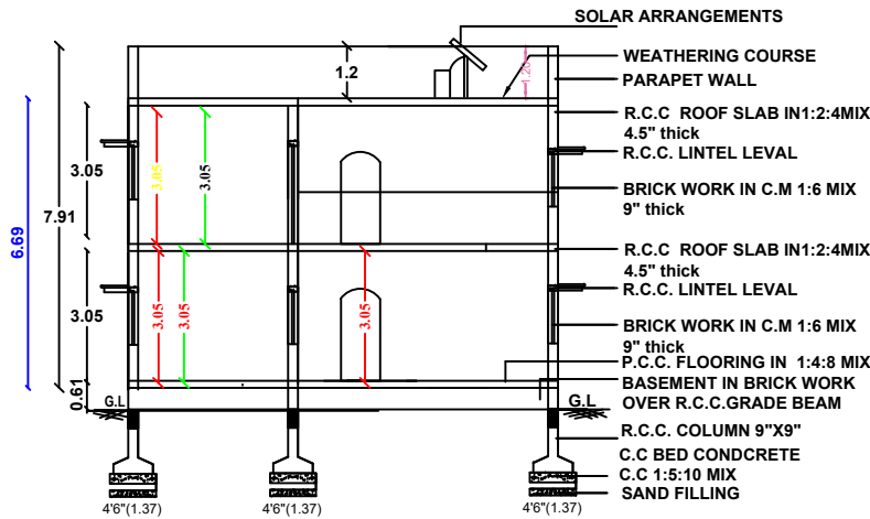
SECTION " AB "
