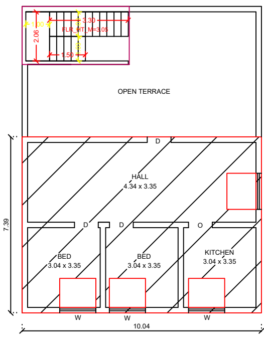
EXG. FIRST FLOOR PLAN
