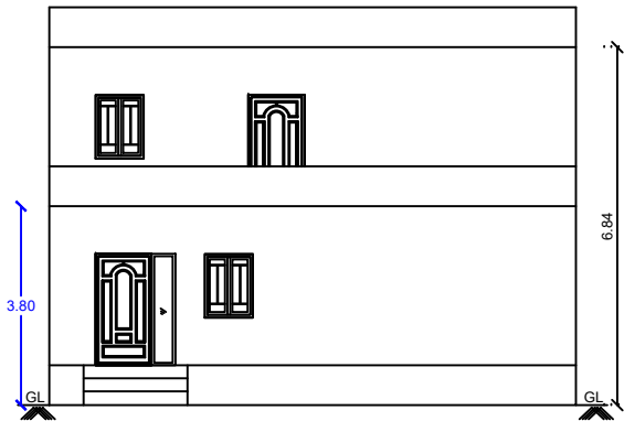
FRONT ELEVATION (NORTH FACING)
