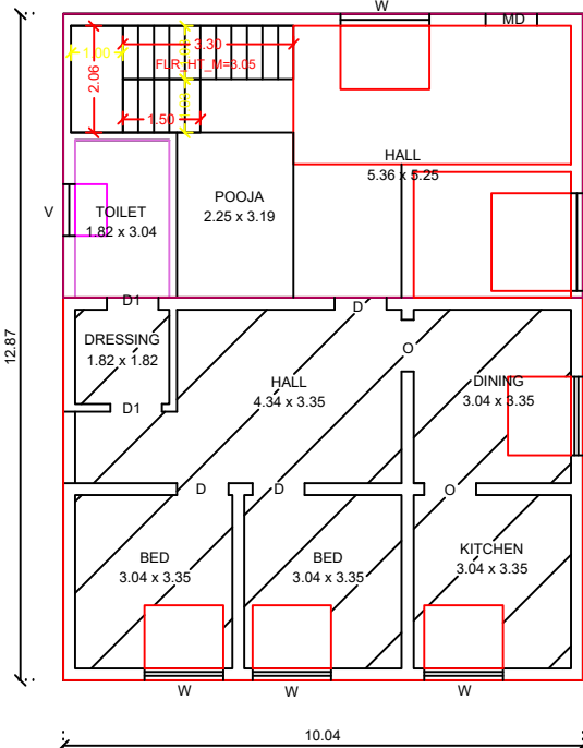
PRO. ADDITIONAL GROUND FLOOR PLAN
