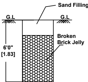
RAIN WATER HARVESTING RECHARGE PIT DETAILS (NOT TO SCALE)
