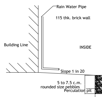
FOUNDATION DETAILS
