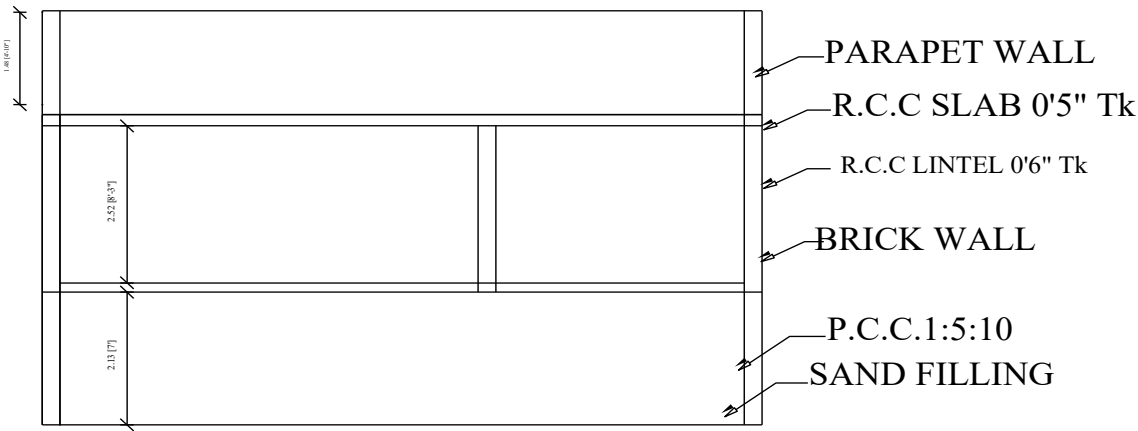
SECTION ON"AB"
