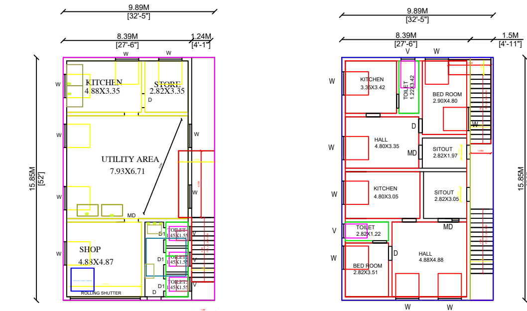
ROPOSED FIRST FLOOR PLAN RESIDENTIAL BUILDING)
