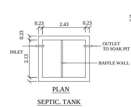
PLAN SEPTIC TANK
