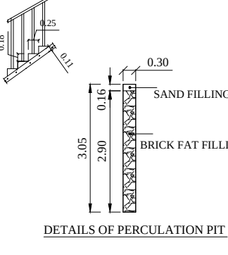
DETAILS OF PERCOLATION PIT
