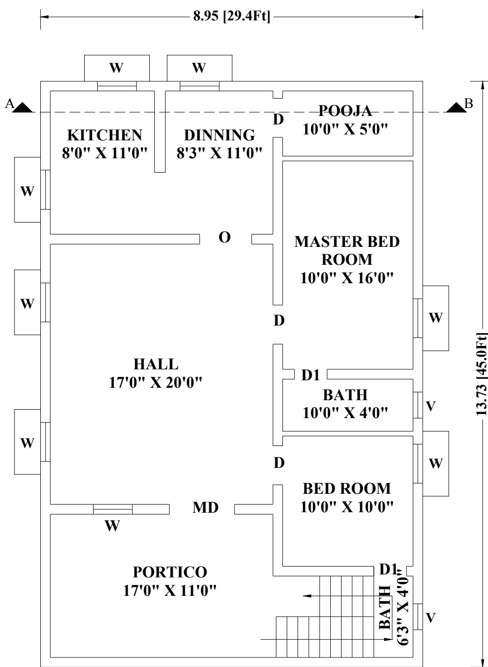
GROUND FLOOR
