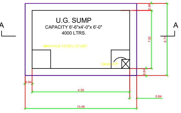
SUMP DETAIL
