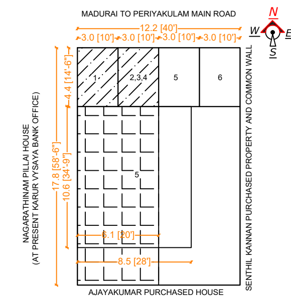
KEY/SITE PLAN FOR SUR. NO. 480/1, 480/2A, 490/2B1A
