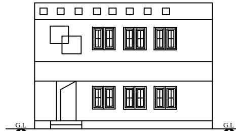
FRONT ELEVATION
