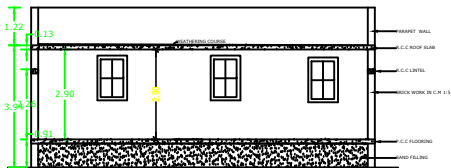
SECTION ON K-S
