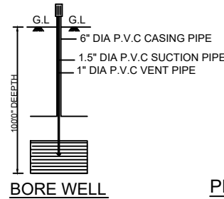
BORE WELL
