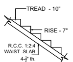
STAIRCASE DETAILS (NTS)
