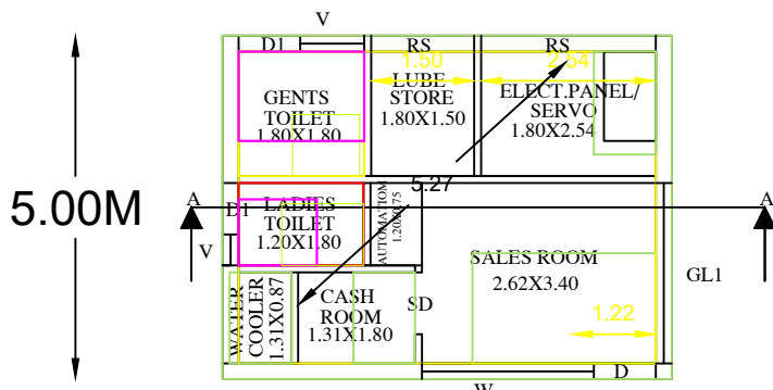
PRO.GROUND FLOOR PLAN
