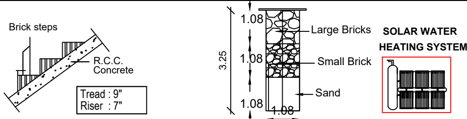
STAIRCASE DETAILS
