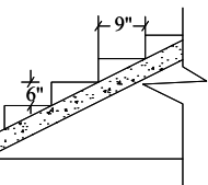
Staircase Detail Not To Scale
