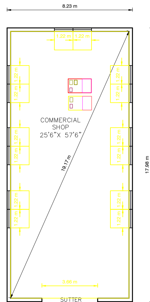
GROUND FLOOR PLAN [SOUTH FACING]
