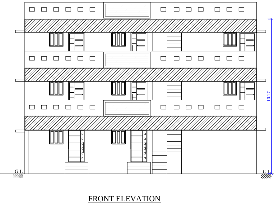
FRONT ELEVATION
