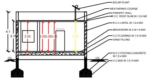
SECTION ON-AA
