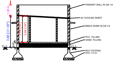
SECTION-"SR"
