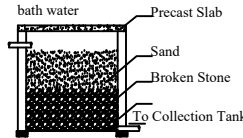
Section of Filter Unit
