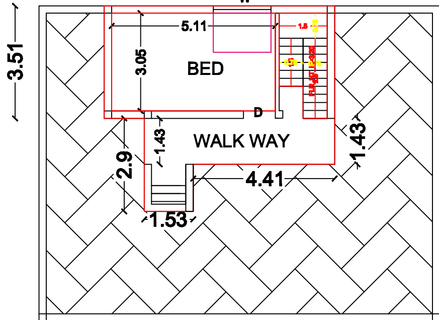
FIRST FLOOR PLAN BLOCK-2
