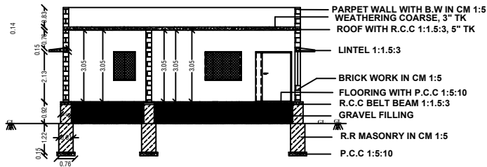
SECTION ON AA' 16.76
