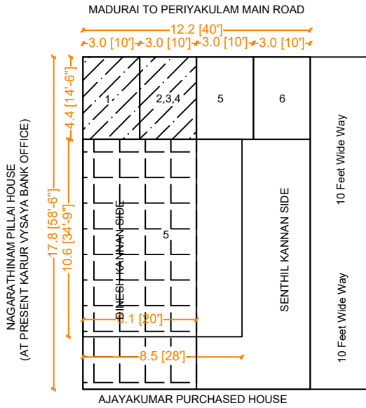
KEY/SITE PLAN FOR SUR. NO. 480/1, 480/2A, 490/2B1A
