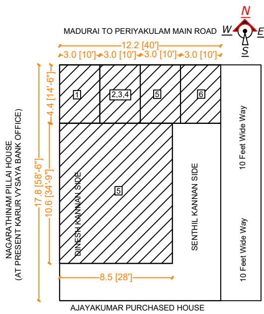
KEY/SITE PLAN FOR SUR. NO. 480/1, 480/2A, 490/2B1A
