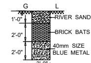
RAIN WATER PERCOLATION PIT (NTS)
