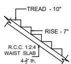
STAIRCASE DETAILS (NTS)
