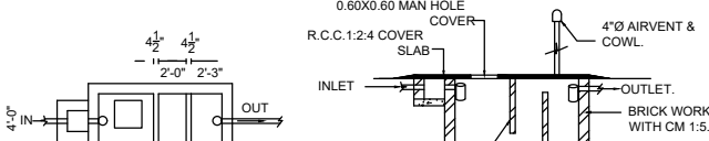
SEPTIC TANK DETAIL
