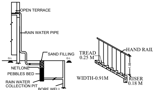
RAIN WATER
