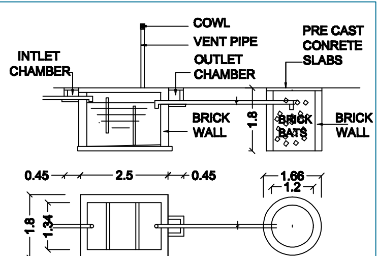
SEPTIC TANK & SOAK PIT
