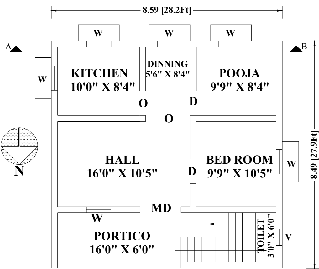
GROUND FLOOR
