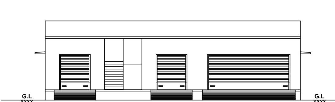
. FRONT ELEVATION .
