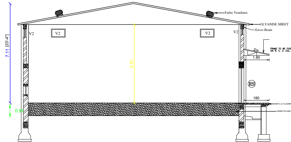
SECTION
