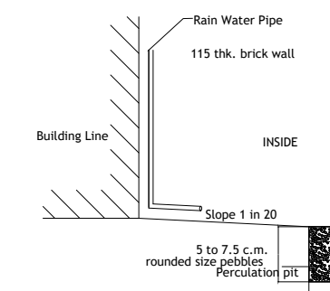
FOUNDATION DETAILS
