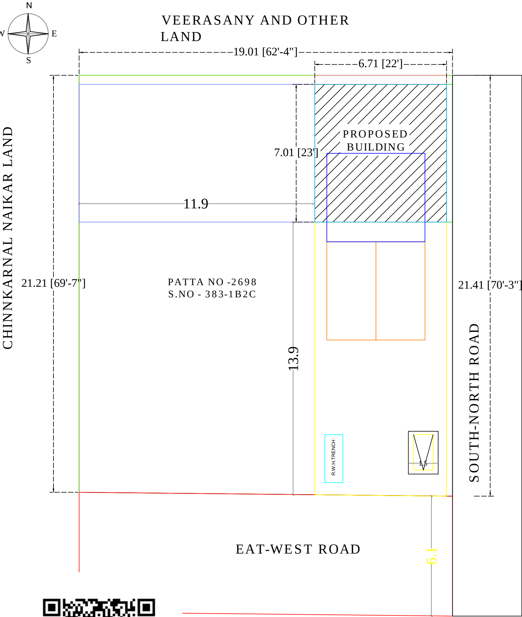
SITE PLAN
