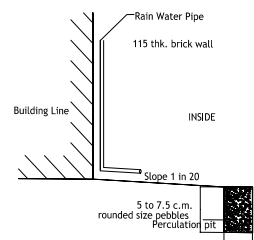
FOUNDATION DETAILS
