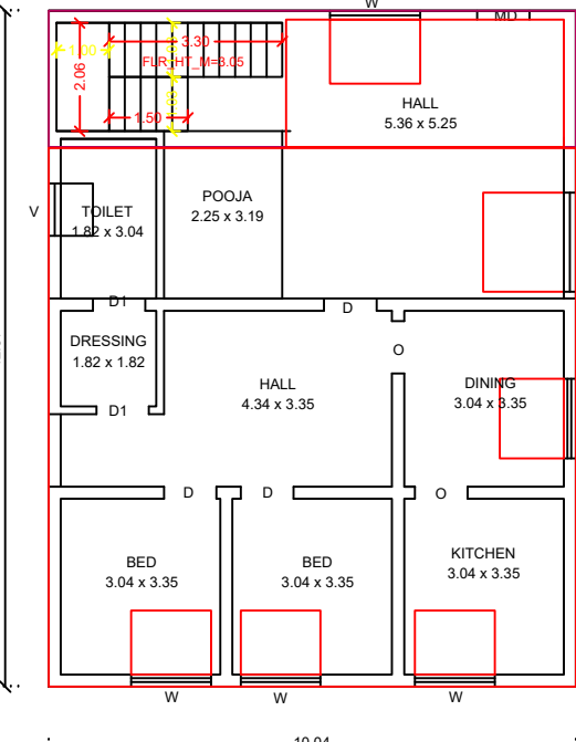
PRO. ADDITIONAL GROUND FLOOR PLAN
