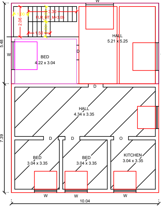
PRO. ADDITIONAL FIRST FLOOR PLAN
