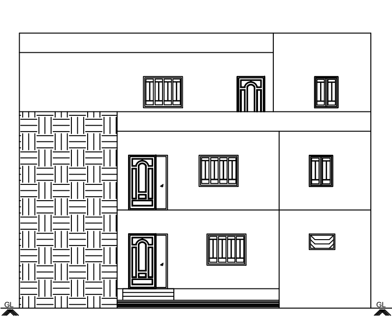
FRONT ELEVATION (EAST FACING)
