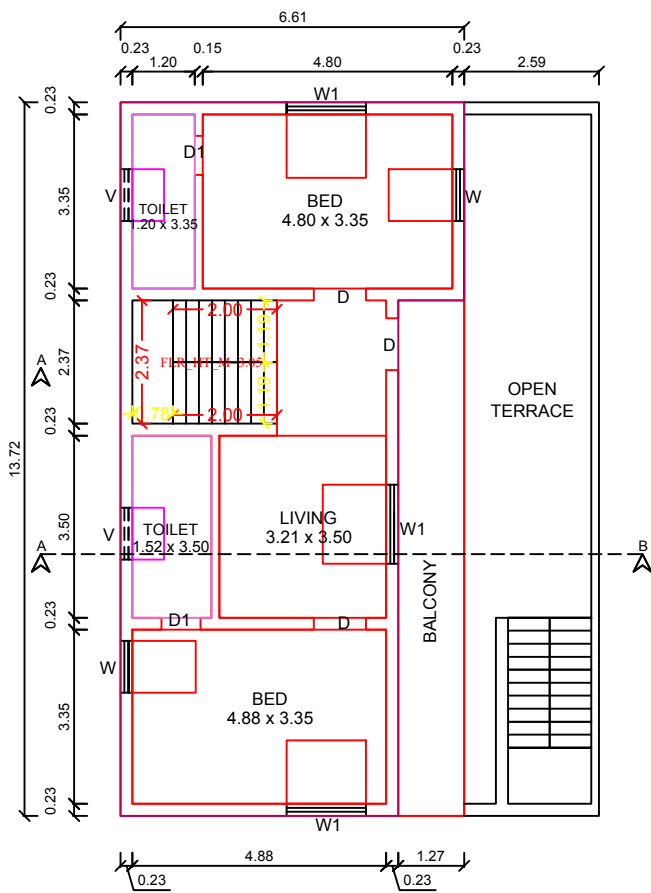
PRO.SECOND FLOOR PLAN
