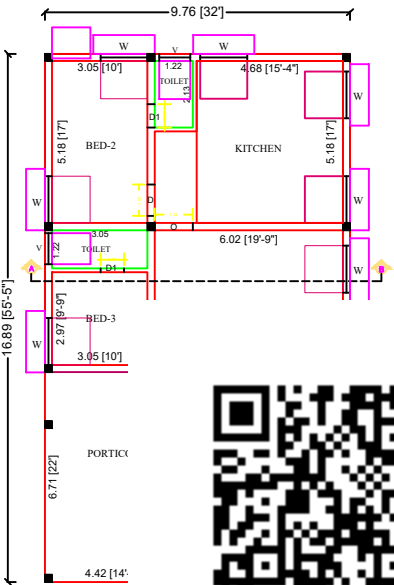
FLOOR PLAN
