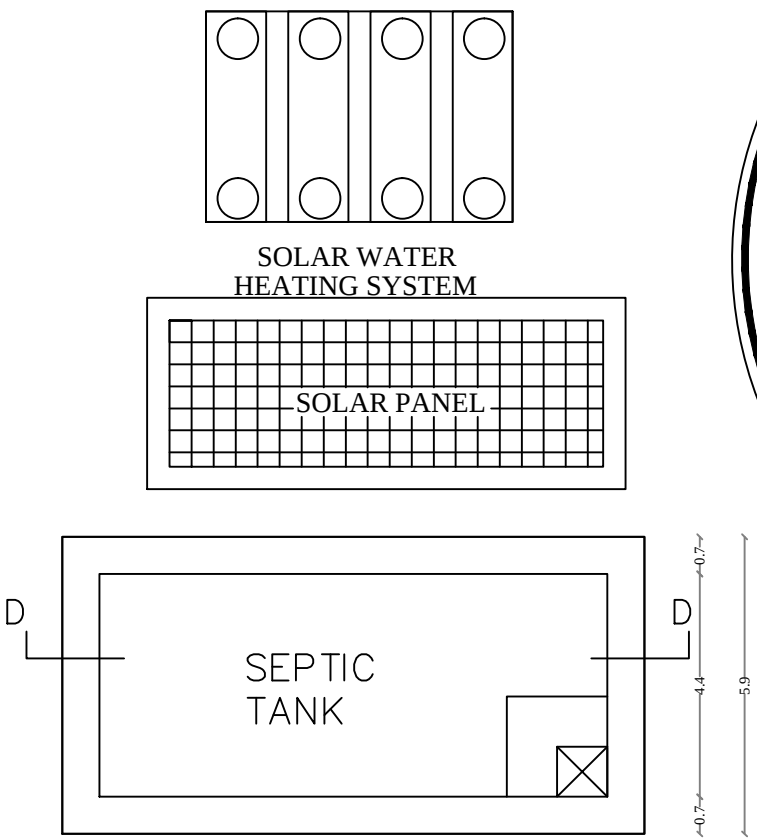
PLAN OF SEPTIC TANK SCALE 1"=2'0"
