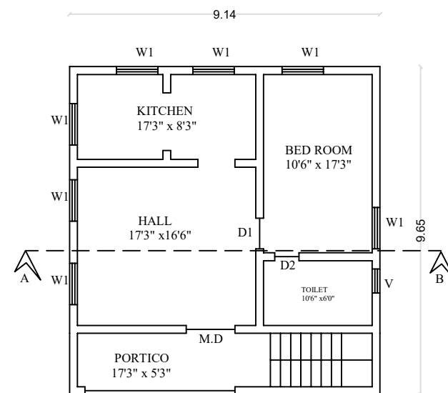
BLOCK-1 GROUND FLOOR PLAN
