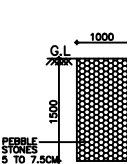
SECTION PEBBLE T SCALE : 1:
