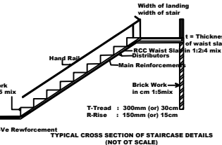
TYPICAL CROSS SECTION OF STAIRCASE DETAILS (NOT TO SCALE)
