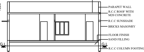
SECTION ON 'SP'
