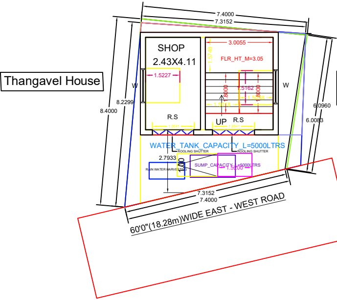
SITE CUM GROUND FLOOR COMMERCIAL PLAN
